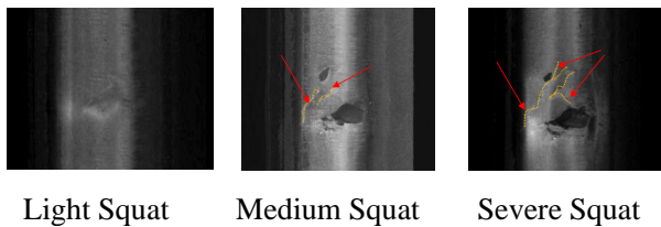
Fig. 3. A sample of squats in different classes of severity, the red arrows show the evolution of the crack when it gets severe.
